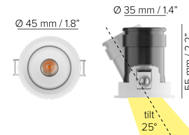
ADJUSTABLE - 6W at 350 mA
