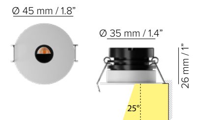
ASYMMETRICAL - 6W at 350 mA
